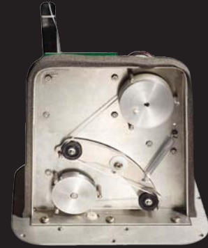
SmartBob-TS1 Mechanical Side
